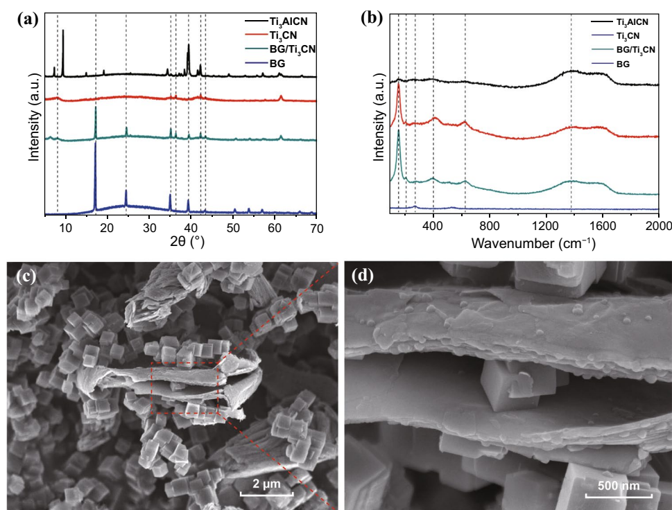
Fig. 5 a XRD patterns and b Raman spectra of Ti 3 AlCN, Ti 3 CN, BG, and BG/Ti 3 CN (1:1). c, d FESEM images in a different amplification of BG/Ti 3 CN BG/Ti 3 CN (1:1)
