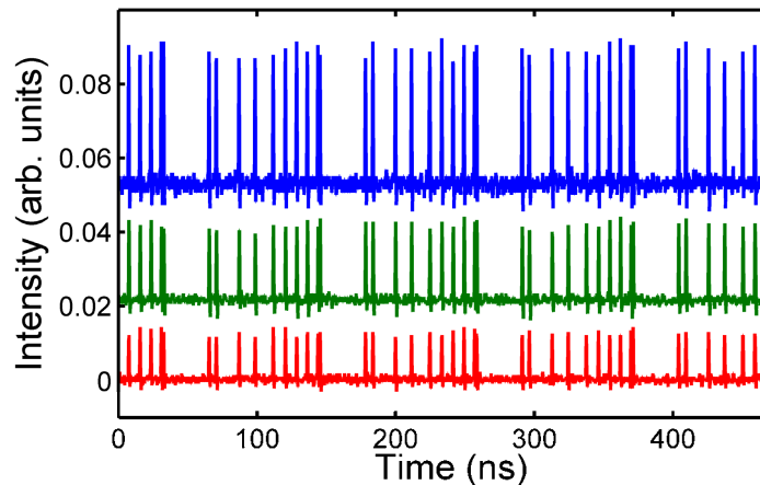
Fig. 3. Oscilloscope traces of the pulse train in a phase locked vector soliton operation state. Blue line: the total laser emission without passing through a polarizer; Red and Green lines: the two orthogonal polarization components resolved with an external cavity polarization beam splitter.
