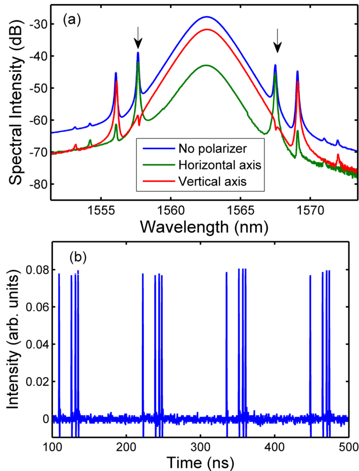
Fig. 2. Vector soliton emission of the fiber laser. (a) Soliton spectra. Blue line: the total laser emission without passing through a polarizer; Red and Green lines: the two orthogonal polarization components resolved with an external cavity polarization beam splitter. (b) Oscilloscope trace of the solitons.
