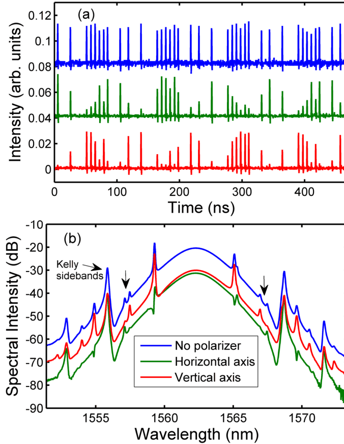
Fig. 4. A polarization rotation vector soliton state of the laser. (a) The total and the polarization resolved soliton pulse trains with multiple solitons in cavity. (b) Optical spectra of the solitons. Blue line: the total laser emission without passing through a polarizer; Red and Green lines: the two orthogonal polarization components resolved with an external cavity polarization beam splitter.
