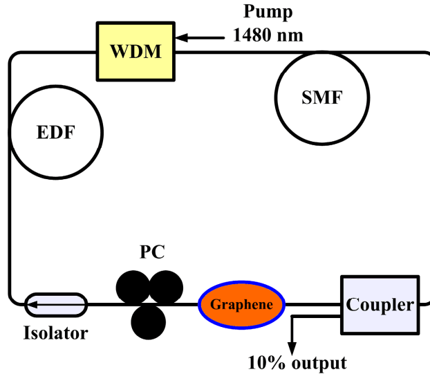
Fig. 1. A schematic of the experimental setup. PC: Polarization controller, EDF: Erbium doped fiber, SMF: Single-mode fiber, WDM: Wavelength-division multiplexer.
